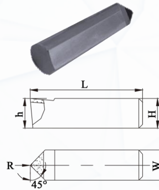
PCD Boring Tool
