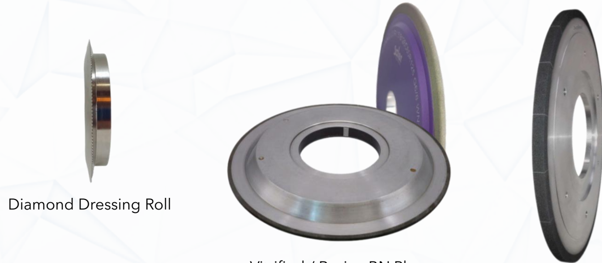
Vitrified / Resin cBN Plunger Grinding Wheel
