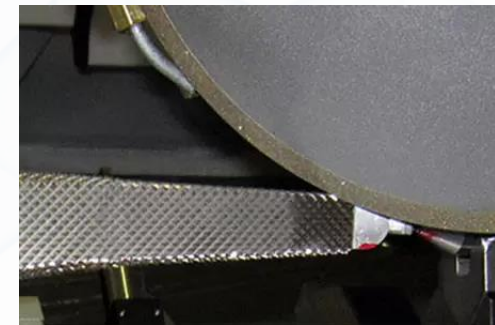
Rasp Grinding - Electroplated Wheel
