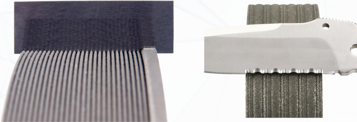
Electroplated cBN wheel for Serration and Edge grinding
