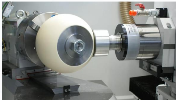
Hip Joint Implant Grinding - Metal Bond Diamond Wheel
