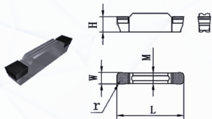
Square Tipped PCD/PcBN Grooving Cutters
