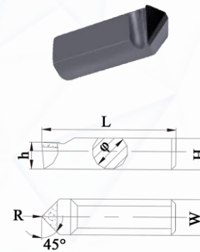
PCD External Turning/Boring Tool
