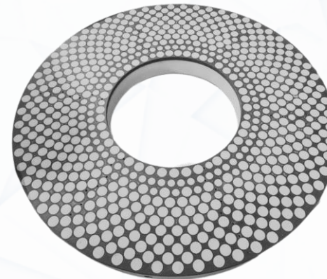
Double Disc Thickness Grinding Wheel
