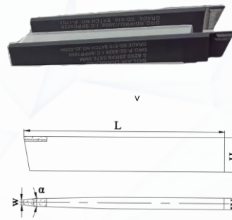
PCD Wedge / rectangle Grooving Tool
