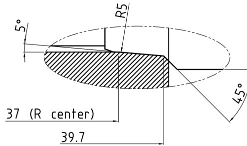
Detail Chamfer Scale (5:1)
